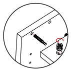
Cam Dowel Assembly
