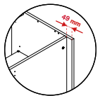
Service void to allow for plumbing, electrics and ventilation
